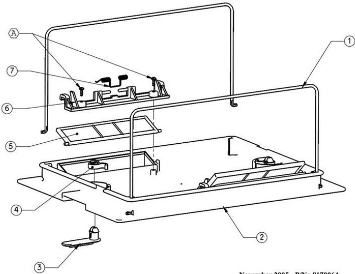
#29 (bottom lid assy db & support)
