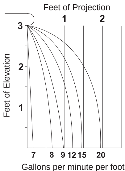
Sheer Descent® Water Flow Requirement Chart
