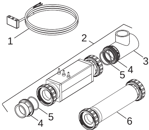
Cell with 1 1/2" Unions
