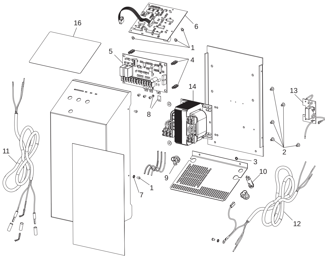
LM2 Series Power Pack
