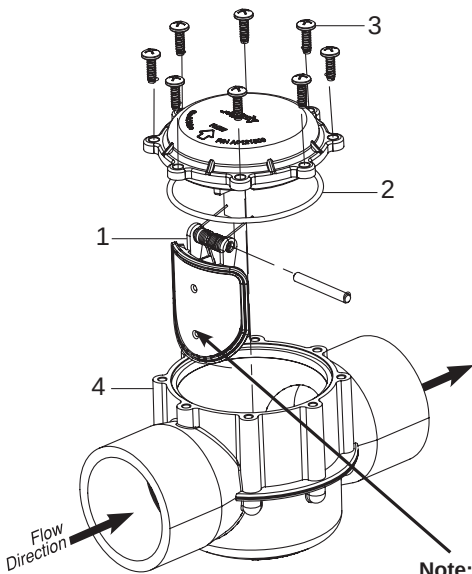
180° Valve Housing OR
