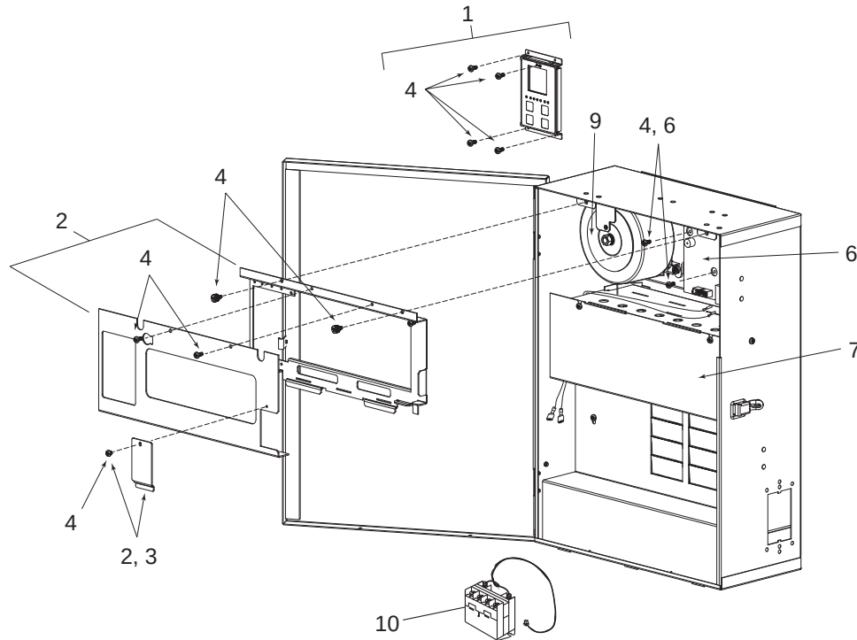
Sub Panel Enclosure
