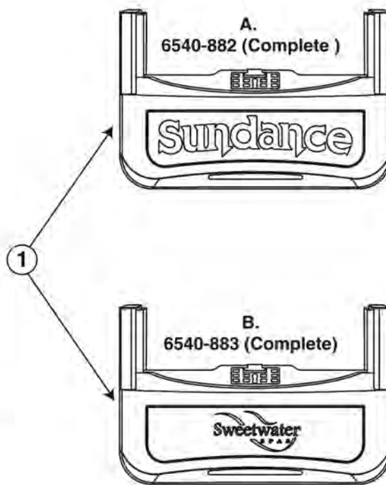
Weir Assembly (Front)
