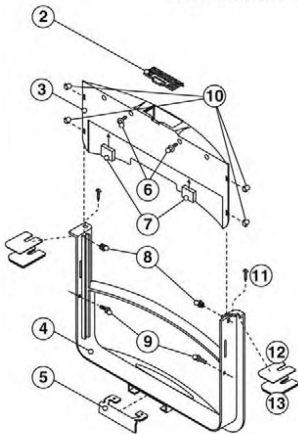
Weir Assembly (Back)
